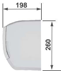
For ASYG07/09/12LE
